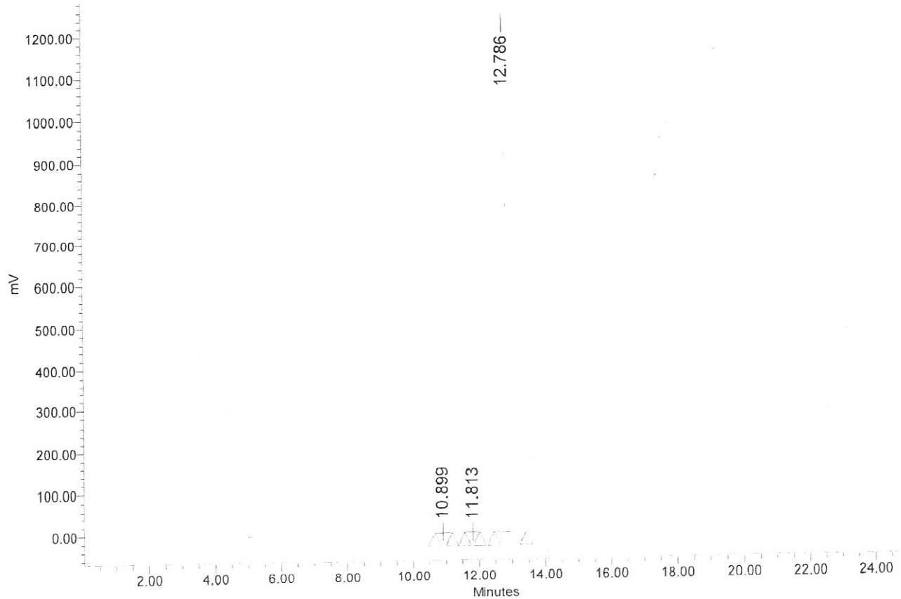
Auto-Scaled Chromatogram
